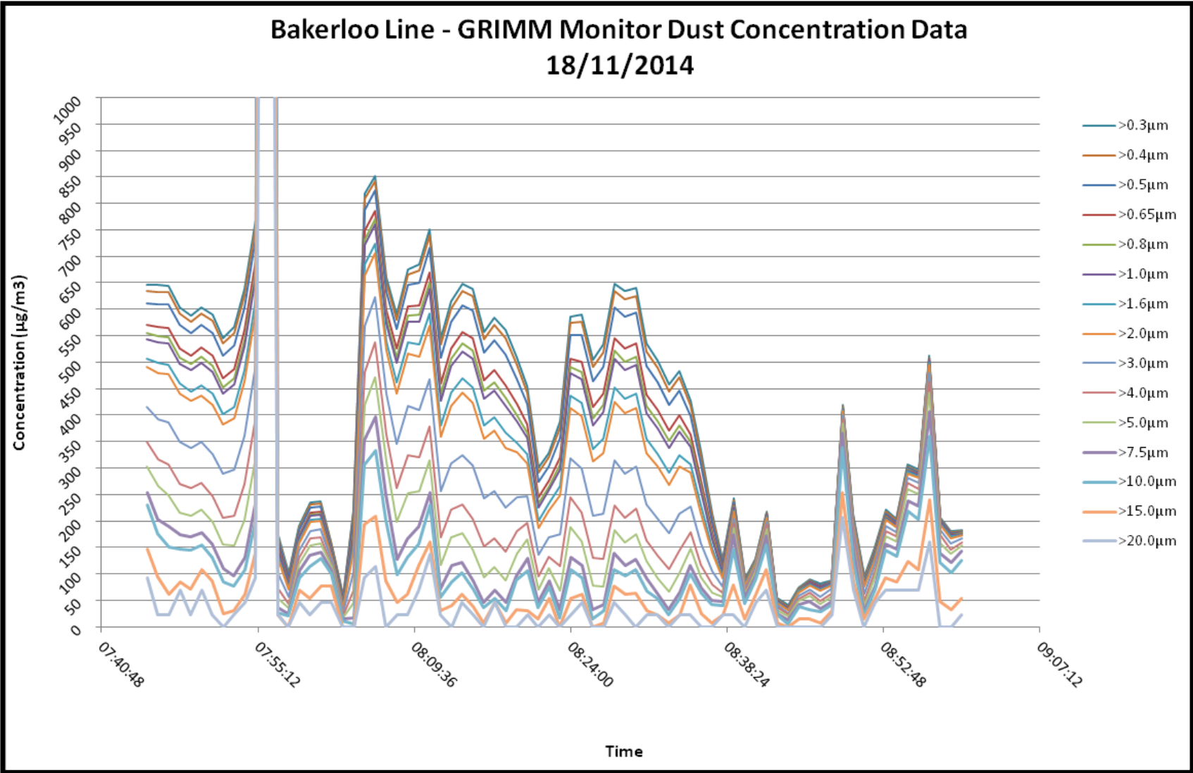
Figure 1: GRIMM monitor dust concentration data at the Bakerloo line on the 18 th November 2014.
