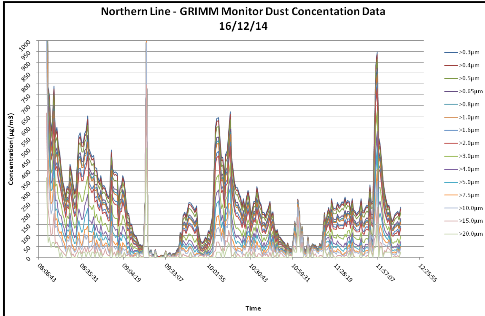
Figure 6: GRIMM monitor dust concentration data at the Northern line on the 16 th December 2014.
