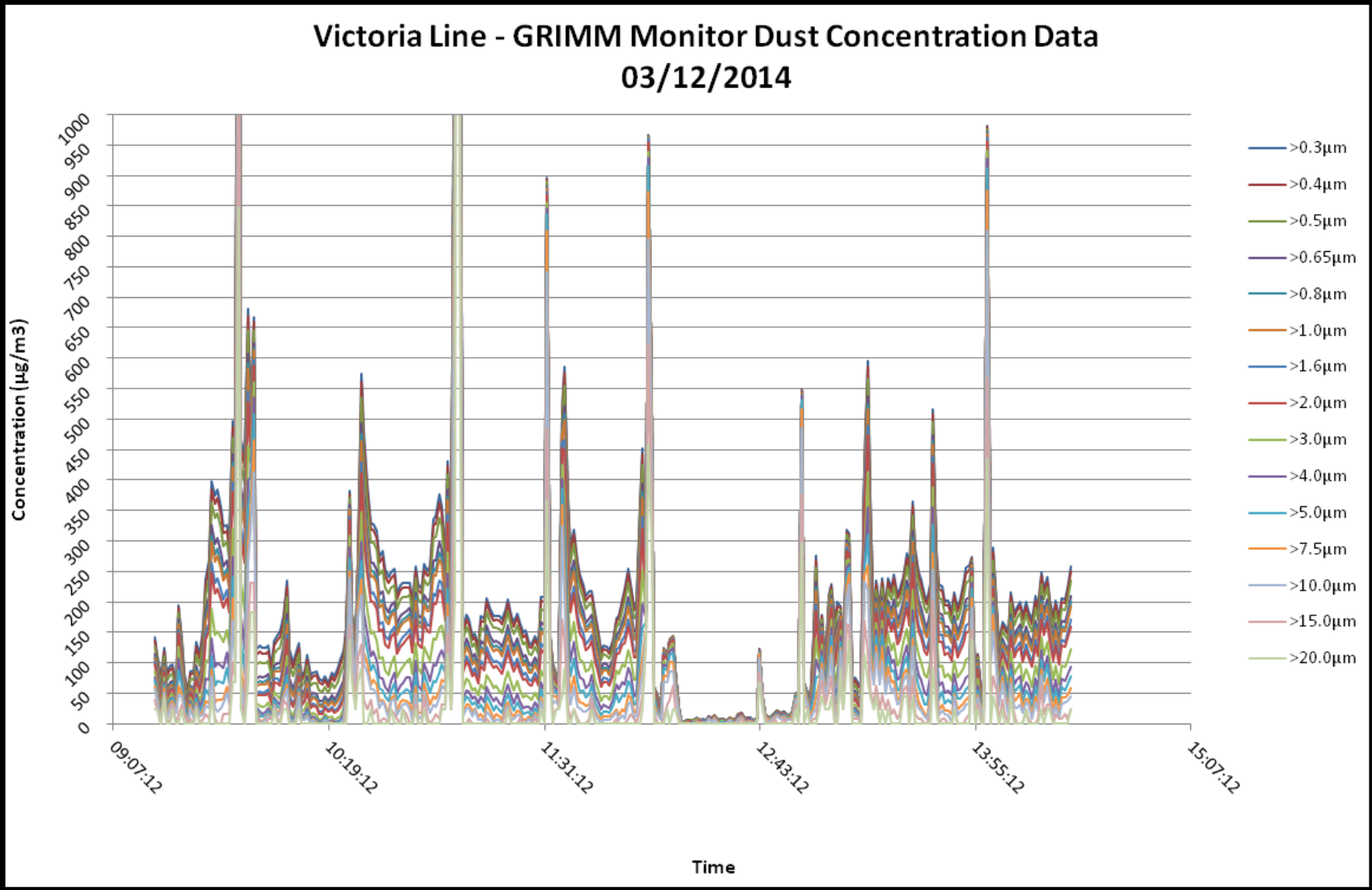
Figure 8: GRIMM monitor dust concentration data at the Victoria line on the 3 rd December 2014.
