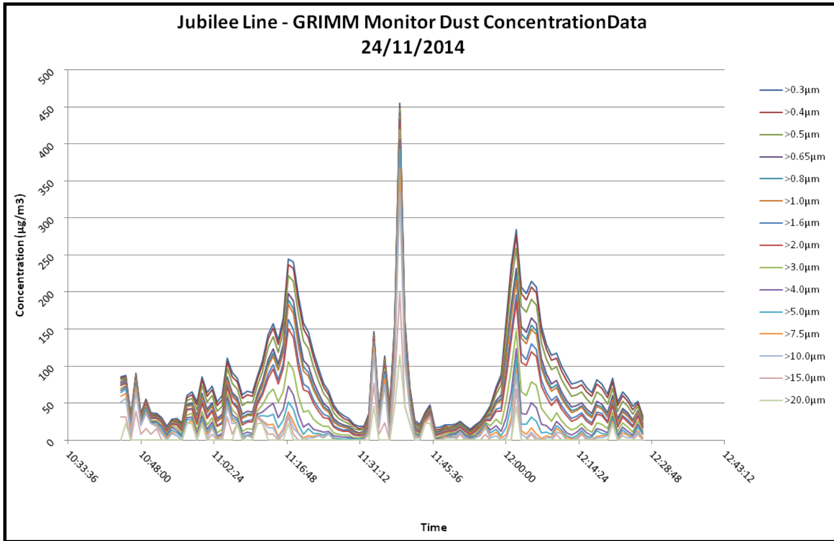
Figure 5: GRIMM monitor dust concentration data at the Jubilee line on the 24 th November 2014.
