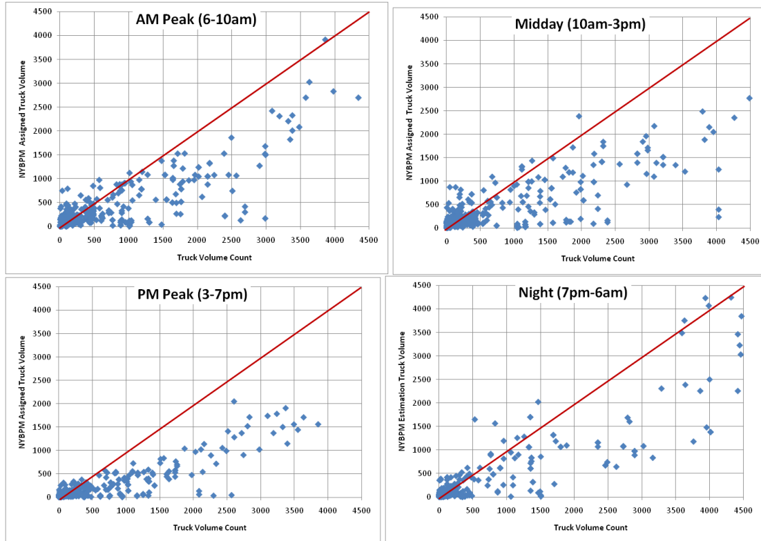
Figure 91: 2007 Truck Volumes vs. BPM Assigned Flows
