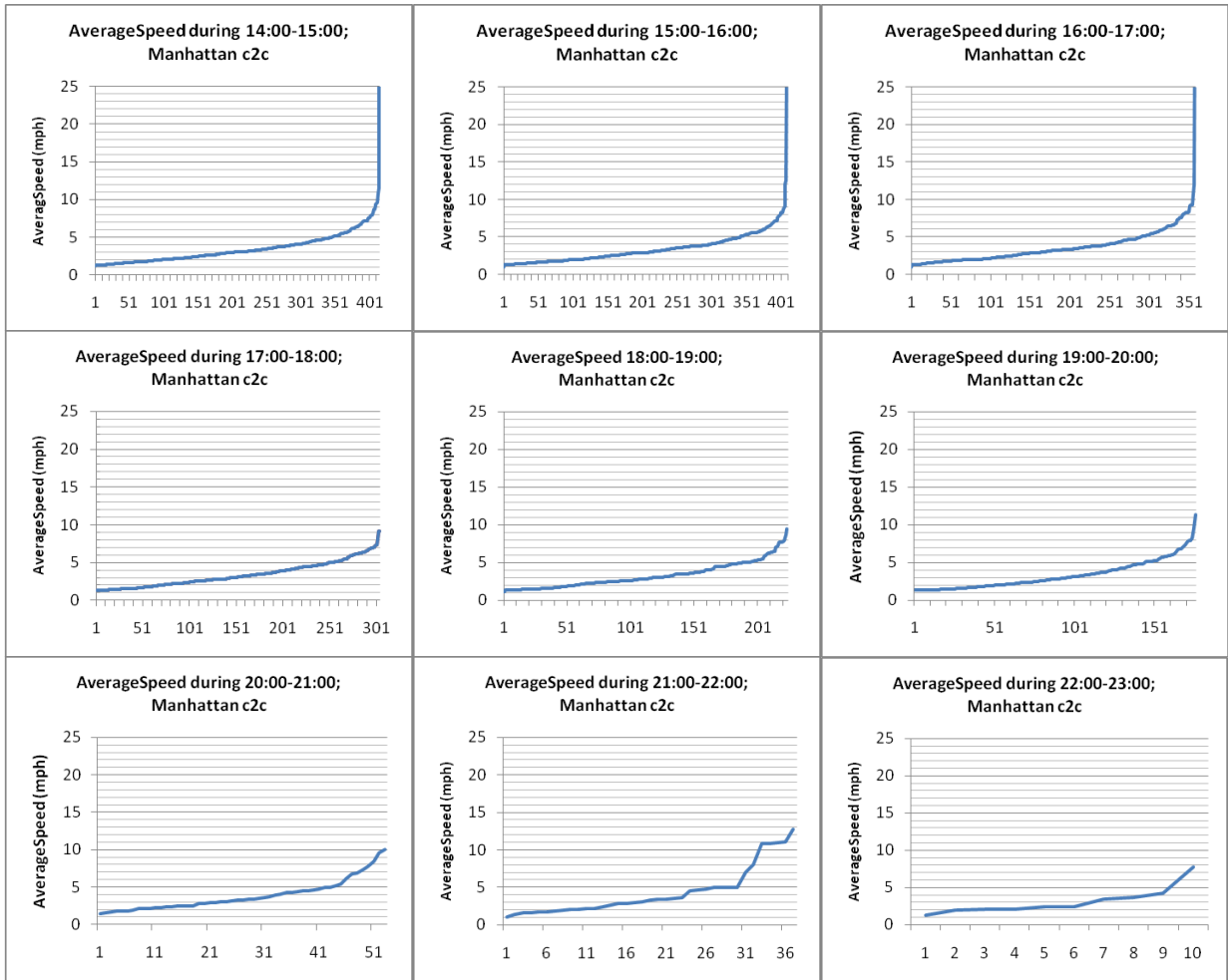
Figure 79: AverageSpeed Distributions for 2 PM to 11 PM - Manhattan c2c Tour Segments
